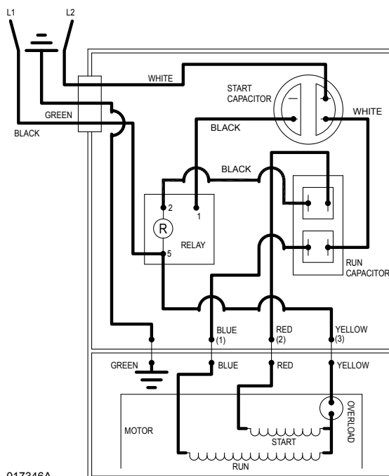
WIRING DIAGRAM FOR MODEL "BN800-A" 12/13 thru Current
