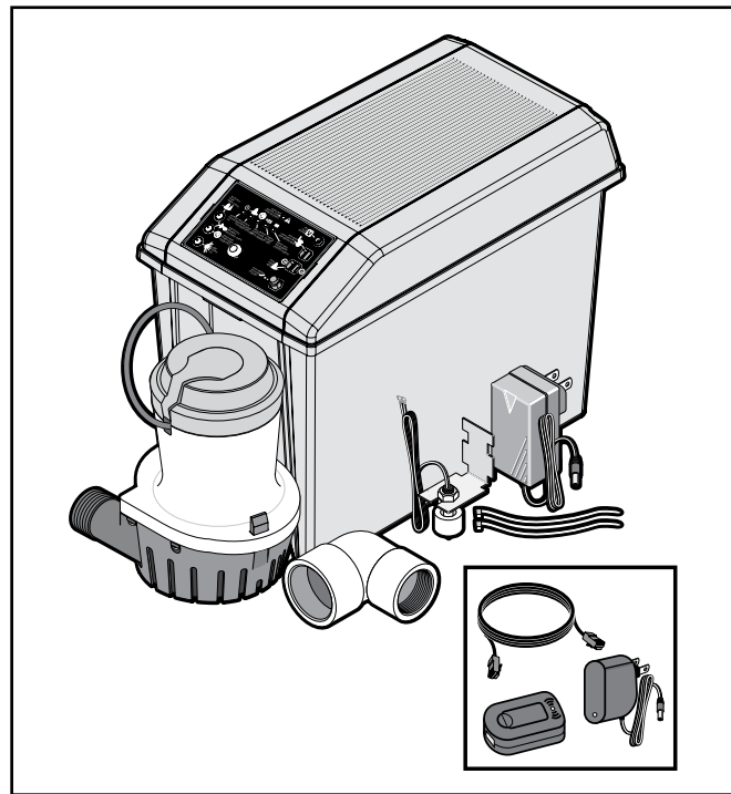
FG-3100RF
