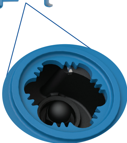
View: Serrated Pump Suction Plate and Mono-Vane Impeller with Steel Cutting Tip
